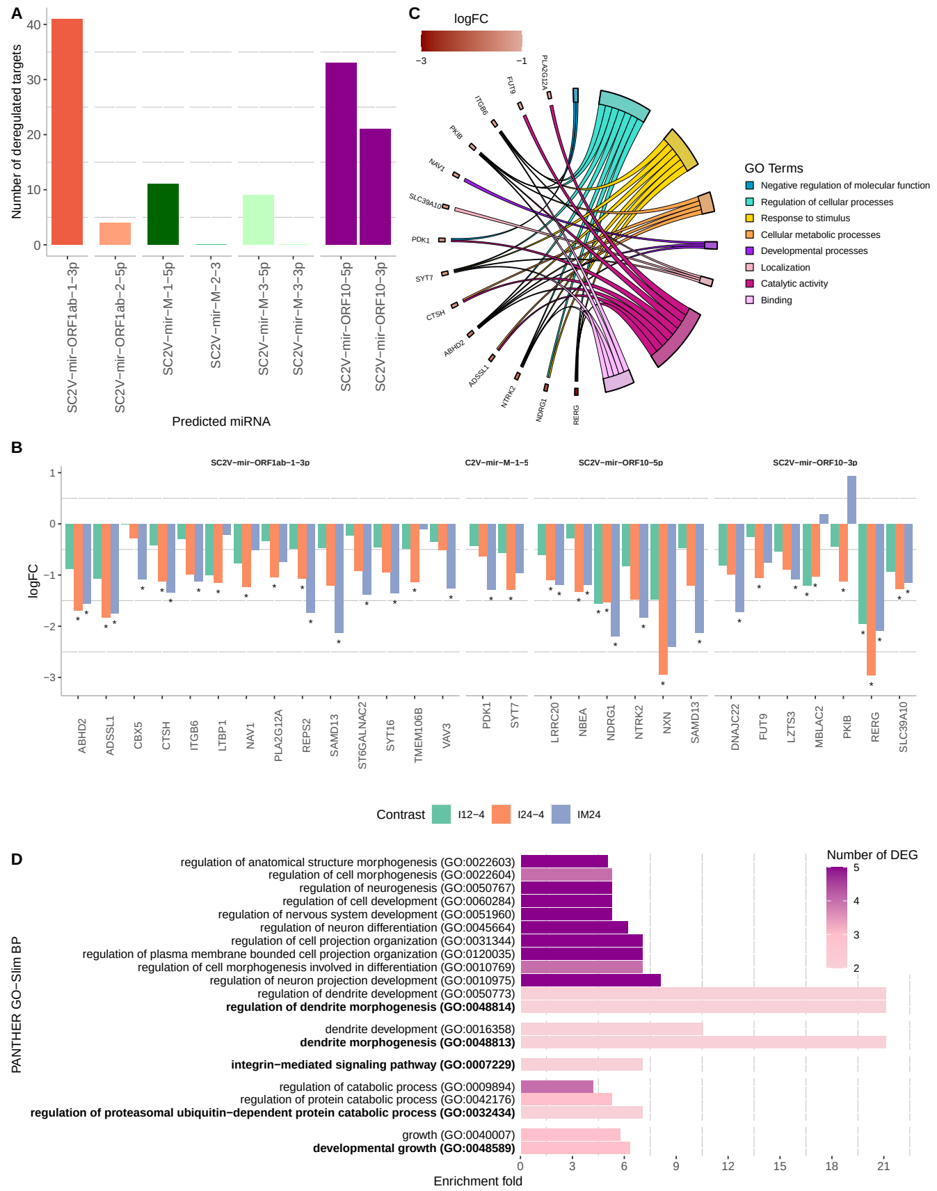
Figure 3: A subset of potential SARS-CoV-2 miRNA targets deregulated upon infection are related to specific biological and molecular functions. A) Number of targets predicted for each SARS-CoV-2 miRNA candidate that were detected as differentially expressed genes (DEGs) in RNA-seq experiments of Calu-3 cultures infected with the virus. Colors indicate the corresponding pre-miRNA. B) Fold change, in log 2 scale, of those predicted SARS-CoV-2 miRNAs targets that were detected as down-regulated in at least one of the contrasts evaluated. Marks indicate significant changes. C) GOChord plot showing Biological Process (BP) and Molecular Function (MF) GO terms of the targets DEGs down-regulated. D) Enrichment results for the overrepresentation analysis of targets DEGs over all the DEGs. Only those BP PANTHER GO-Slim terms with enrichment scores higher than 4.2 (average enrichment score) are shown. Terms are grouped based on the ontology hierarchy being the term in bold the deepest.
