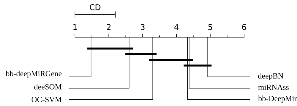
Fig. 2. CD diagram for the pre-miRNA prediction methods along all genome-wide datasets.
